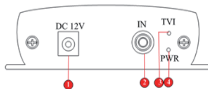
Front Panel
