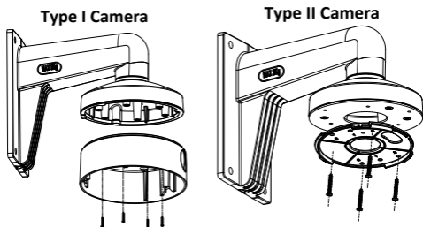
Figure 2-6 Attach the Base Plate to the Bracket
