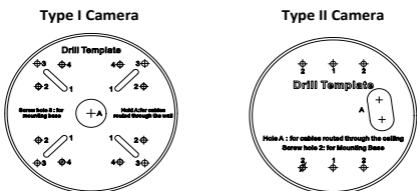
Figure 2-1 The Drill Template
