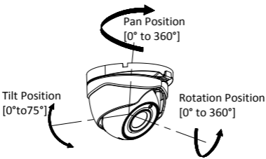
Figure 2-14 3-axis Adjustment
