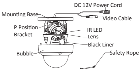
Figure 1-1 Overview of Dome Camera
