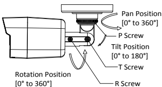
Figure 2-3 3-axis Adjustment
