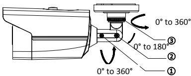
Figure 2-10 3-Axis Adjustment
