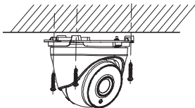
Figure 2-3 Fix the Mounting Base and Camera
