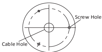
Figure 2-1 Drill Template
