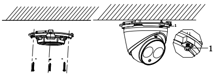
Figure 2-5 Fix the camera to the ceiling
