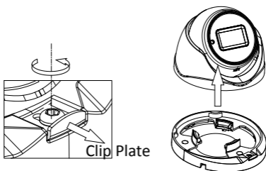
Figure 2-8 Remove the Clip Plate
