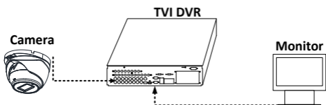
Figure 3-1 Connection
