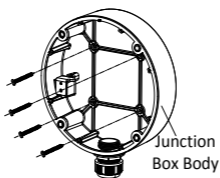
Figure 2-14 Secure the Junction Box's Body on Ceiling
