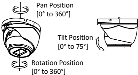
Figure 2-11 3-axis Adjustment
