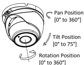
Figure 2-11 3-axis Adjustment
