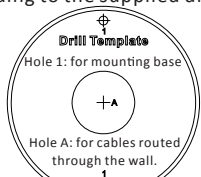
Figure 2-4 The Drill Template
