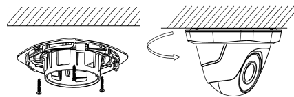
Figure 2-7 Fix the Mounting Base and Camera
