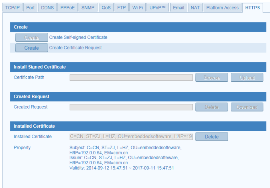
Figure 6-23 HTTPS Settings
