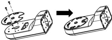
Figure 2-12 Install the Installation Plate
