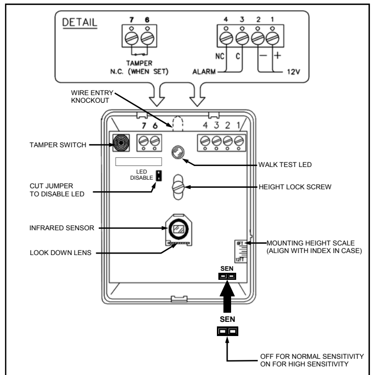
PIR1710 Circuit Board Detail
