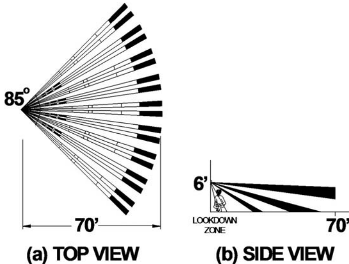
Standard Lens Coverage Pattern
