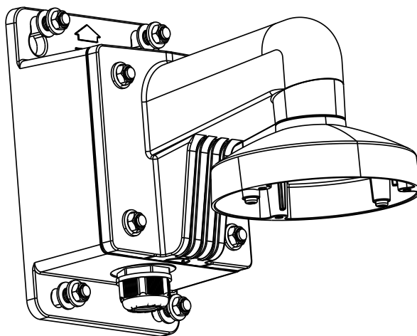
Figure 4-25 Install Wall Bracket
