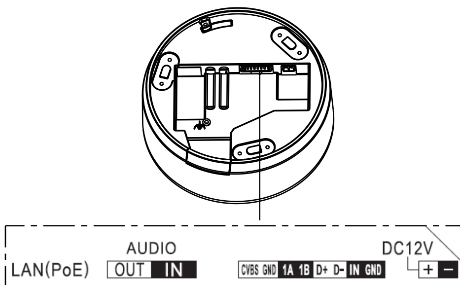
Figure 3-81 Overview (4)
