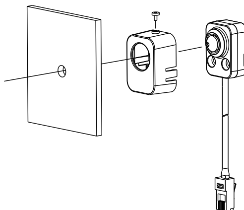
Figure 6-9 Insert the Block-shaped Sensor Unit
