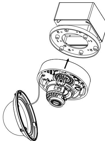
Figure 3-71 Secure Camera
