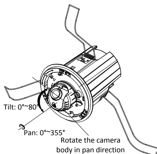
Figure 3-112 Adjust the View Angle
