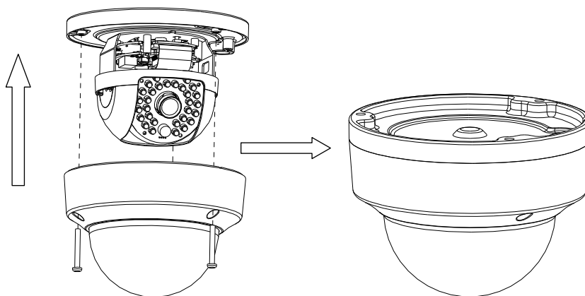
Figure 3-51 Bubble Reinstallation
