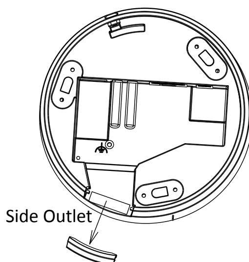
Figure 3-83 Side Outlet
