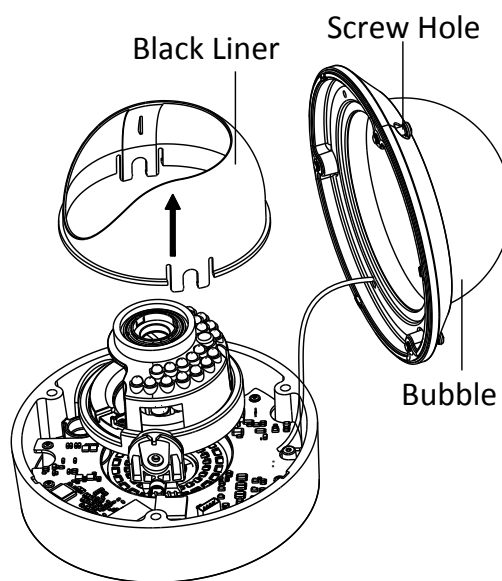
Figure 3-63 Remove the Bubble and Black Liner
