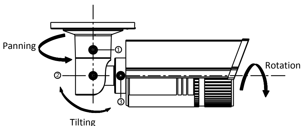
Figure 5-32 Lens Adjustment
