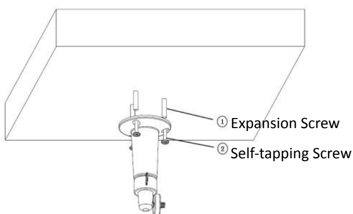
Figure 7-2 Fix the Bracket
