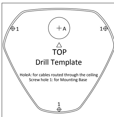
Figure 8-4 Drill Template
