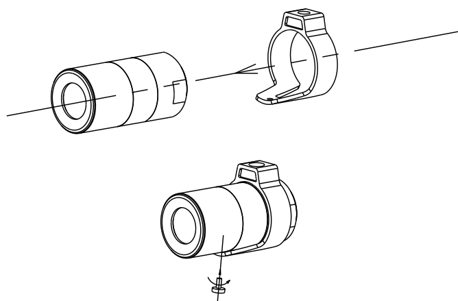
Figure 6-18 Loop the Fixed Focal Unit
