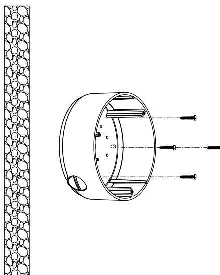
Figure 3-32 Secure Back box
