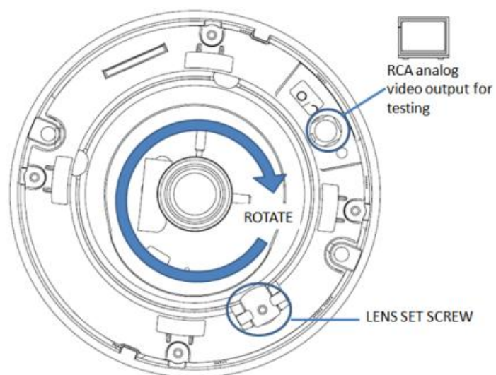
Figure 3-7 Image Adjusting
