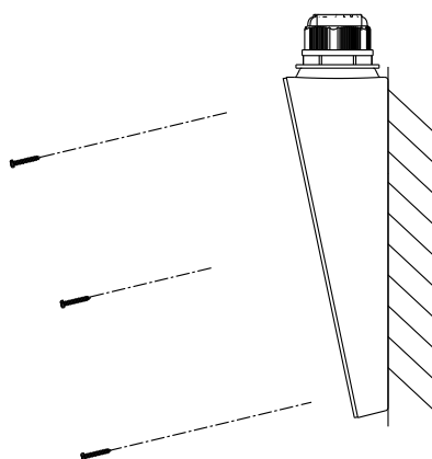
Figure 8-9 Hammer the Screws
