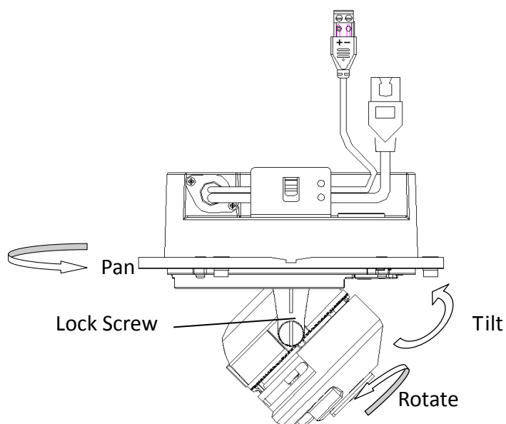
Figure 3-35 Angle Adjusting
