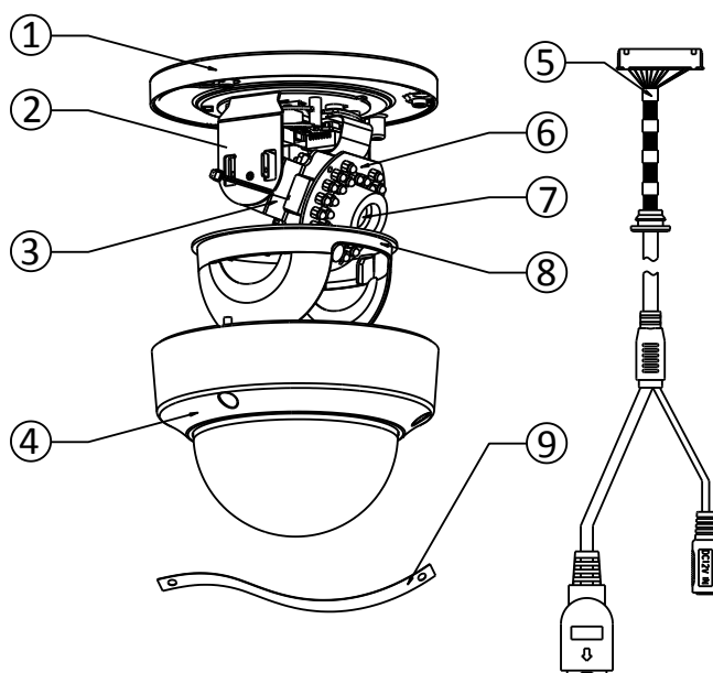
Figure 3-45 Overview
