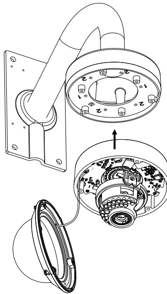
Figure 3-74 Secure Camera
