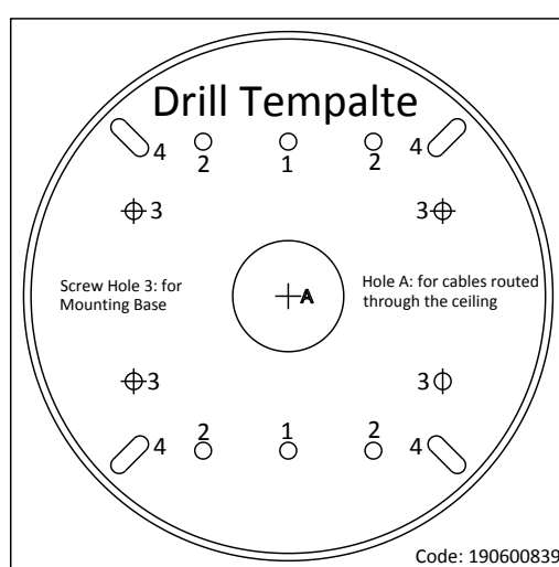
Figure 3-93 Drill Template
