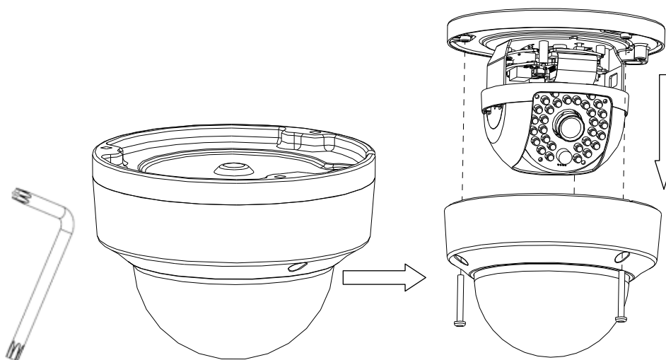
Figure 3-47 Remove the Bubble
