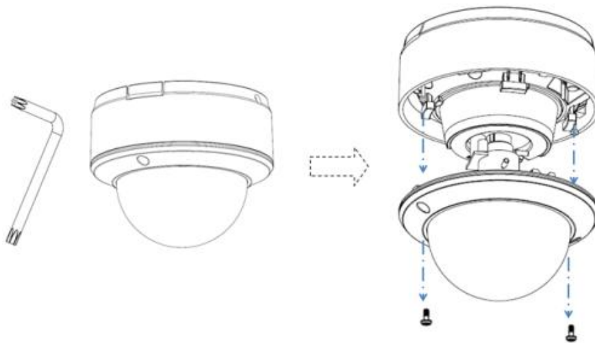
Figure 3-5 Disassembling
