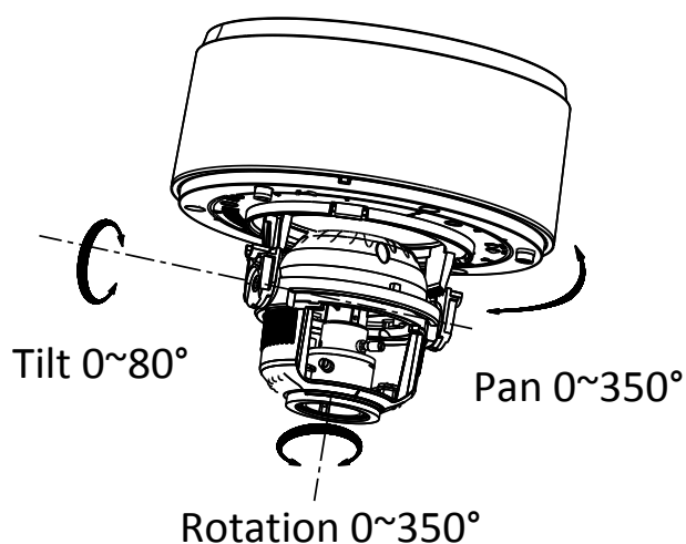
Figure 3-111 3-axis Adjustment
