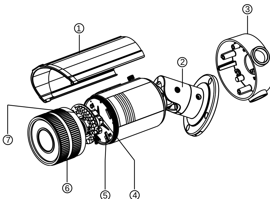
Figure 6-34 Overview
