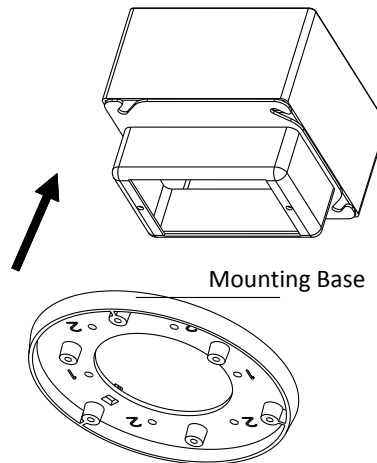
Figure 3-85 In-ceiling Mount
