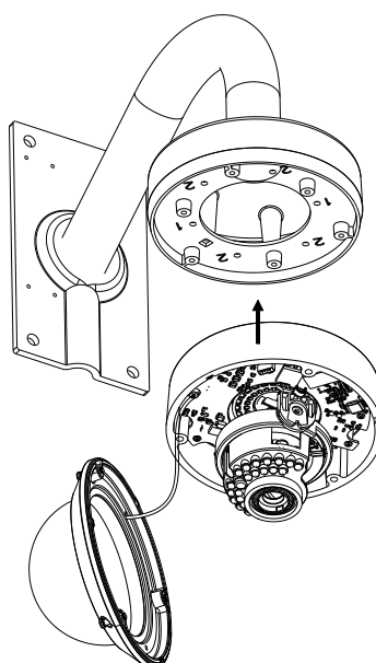
Figure 3-89 Secure Camera
