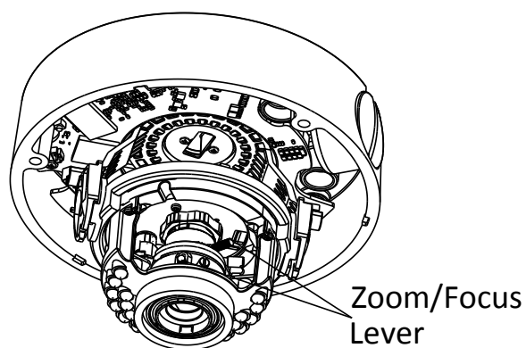
Figure 3-92 Lens Adjustment
