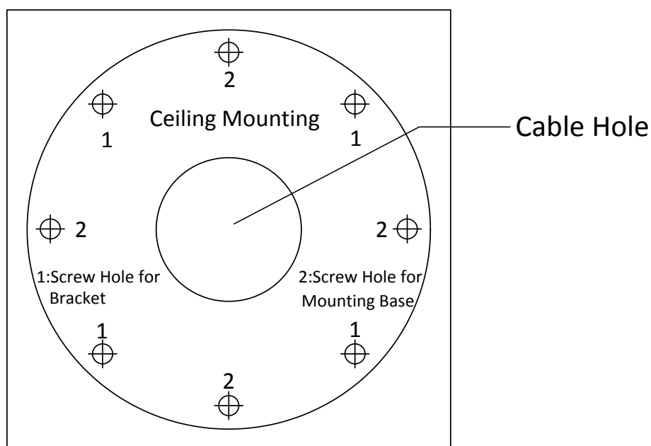
Figure 6-60 Drill Template
