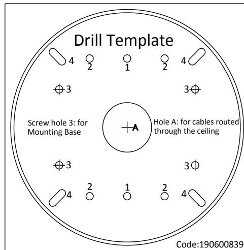
Figure 3-31 Drilling Template
