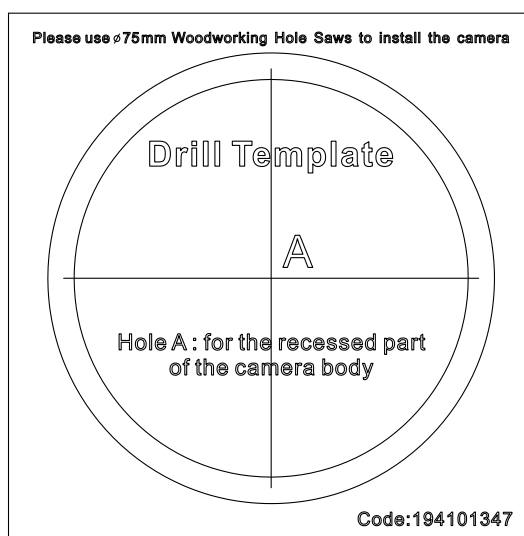
Figure 3-124 Drill Template
