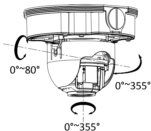
Figure 3-141 3-axis Adjustment
