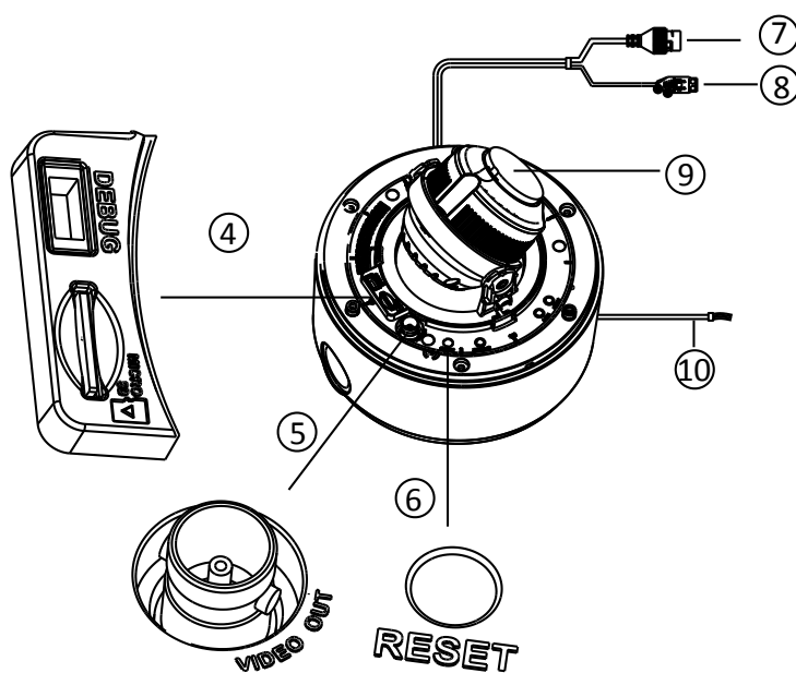
Figure 3-107 Overview (2)
