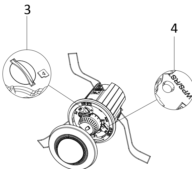
Figure 3-121 Overview(2)
