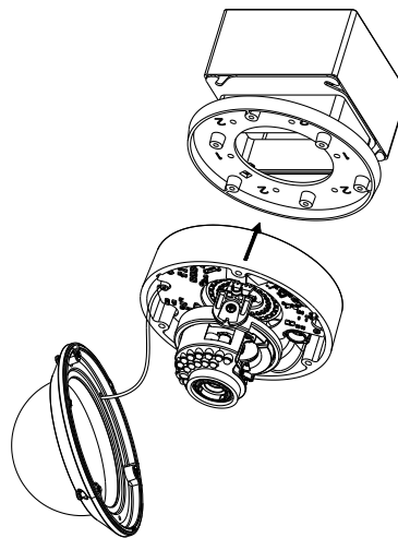
Figure 3-86 Secure Camera
