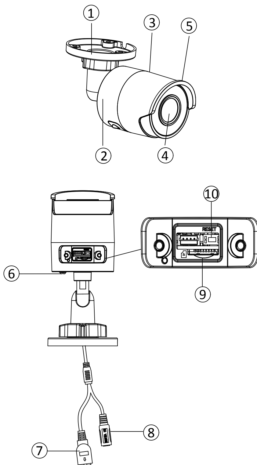
Figure 6-51 Overview
