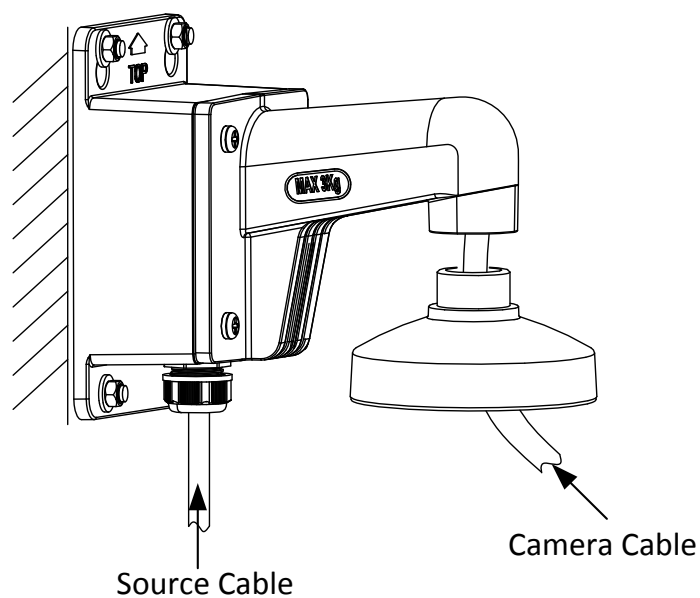
Figure 3-50 Cable Routing
