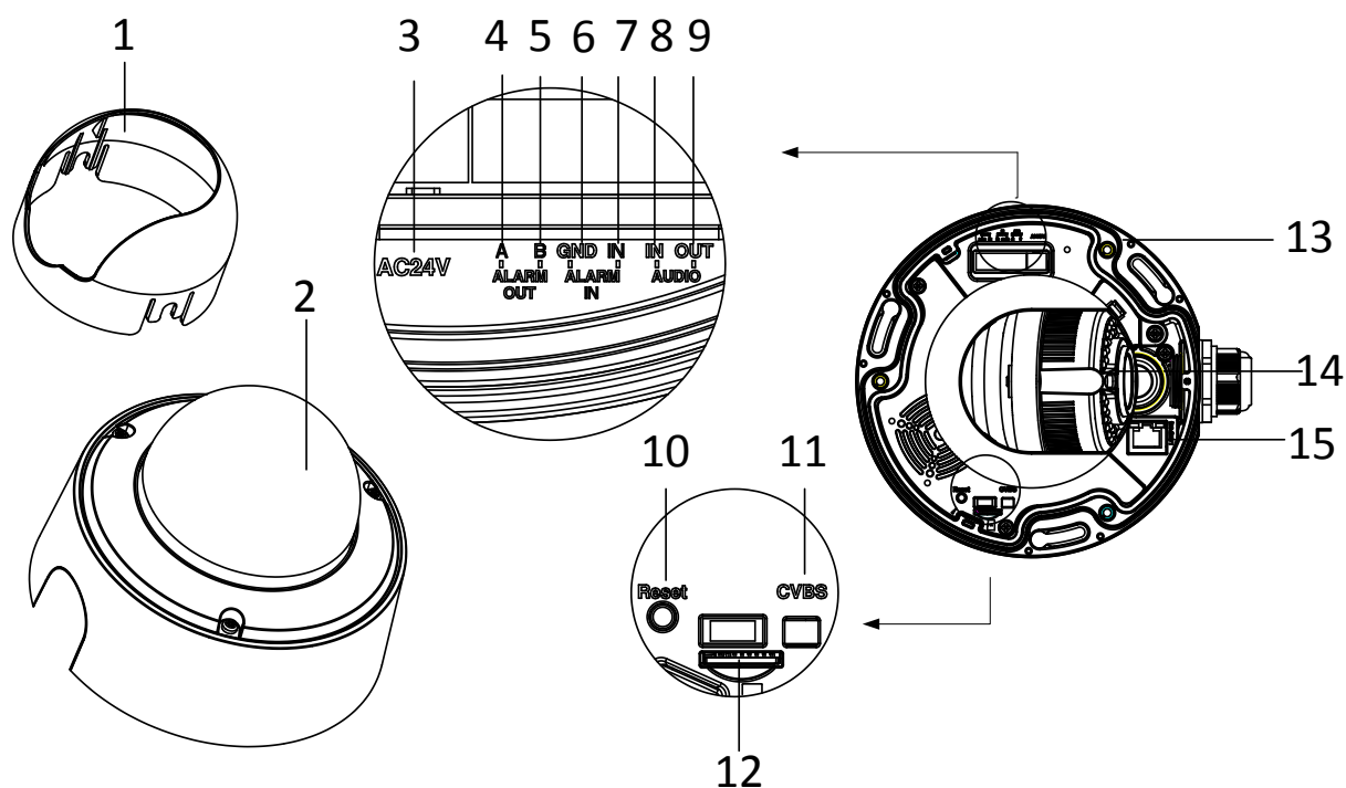
Figure 3-131 Detailed Components
