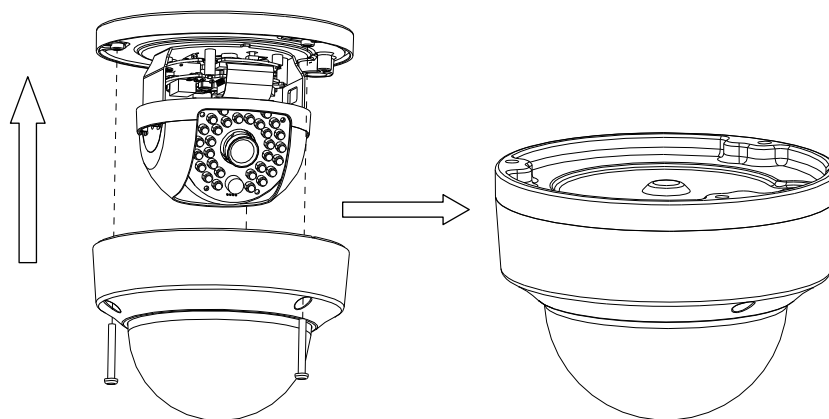
Figure 3-66 Bubble Reinstallation
