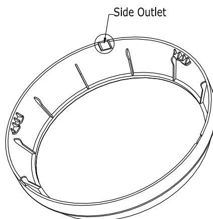
Figure 5-4 Side Outlet
