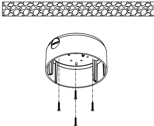
Figure 3-19 Mount Back Box
