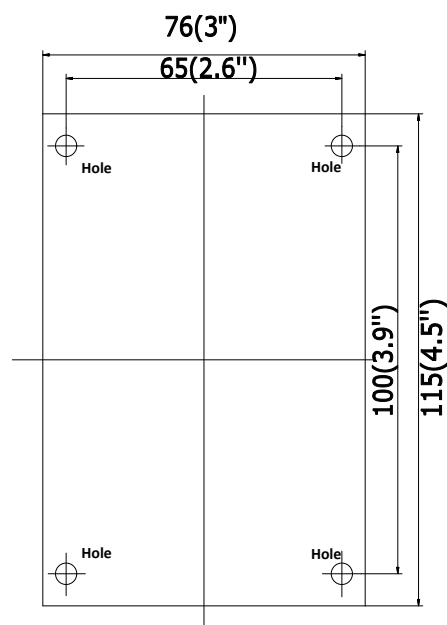
Figure 3-44 Mark Screw Hole
