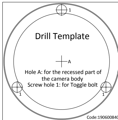
Figure 3-25 Drill Template
