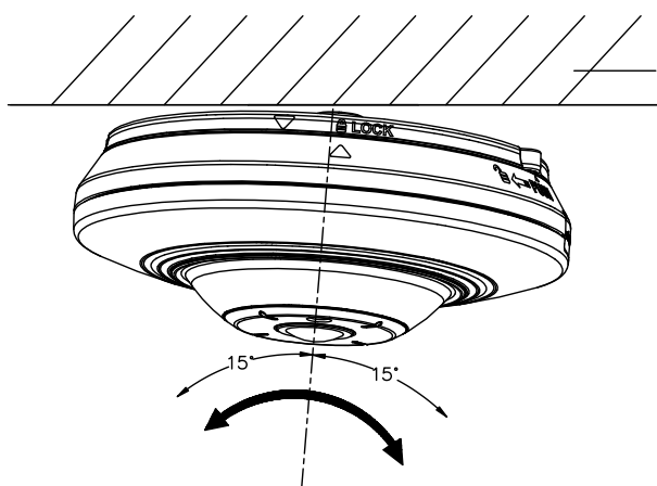
Figure 9-33 Adjust View Angle
