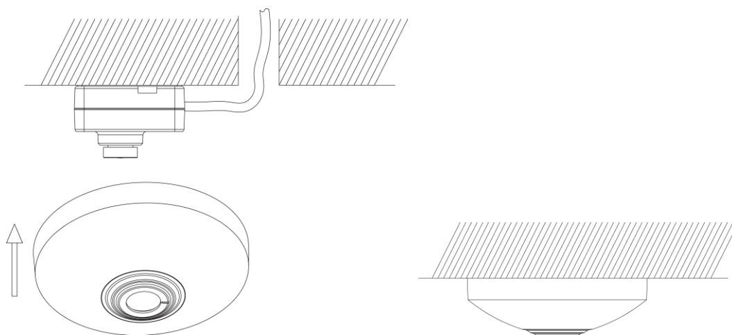
Figure 10-13 Attach the lens cover
