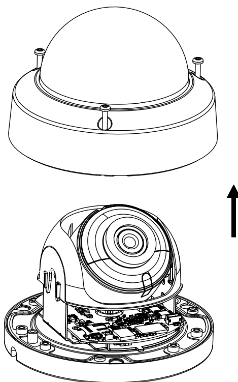
Figure 3-37 Remove Bubble
