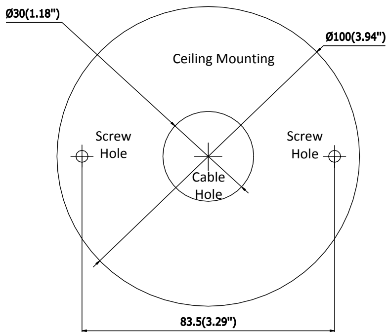
Figure 3-56 Drill Template
