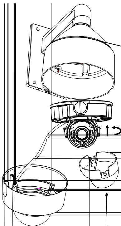
Figure 3-124 Install the Black Liner and Bubble
