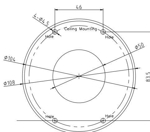
Figure 3-53 Drill Template
