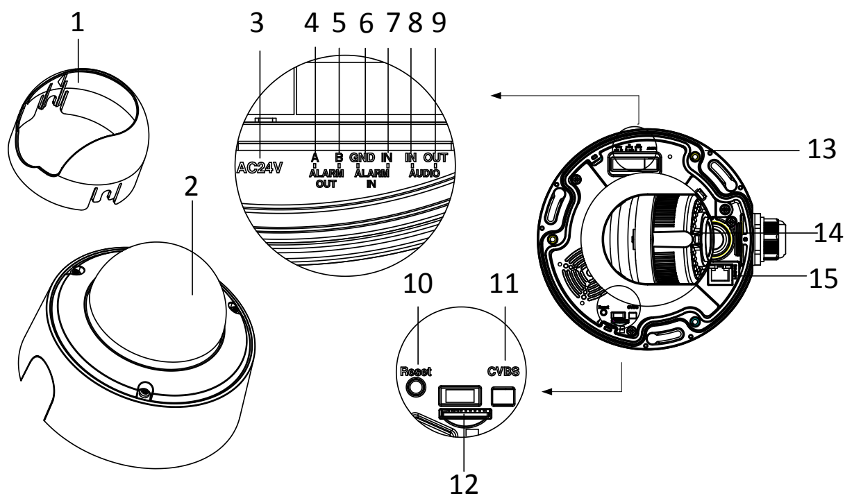
Figure 3-116 Detailed Components
