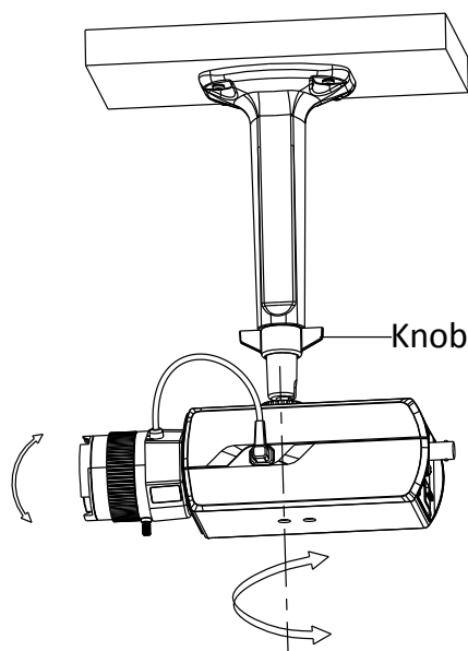
Figure 2-12 Install the Camera to the Mount and Adjust the Angle
