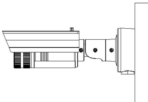
Figure 5-8 Complete the Installation
