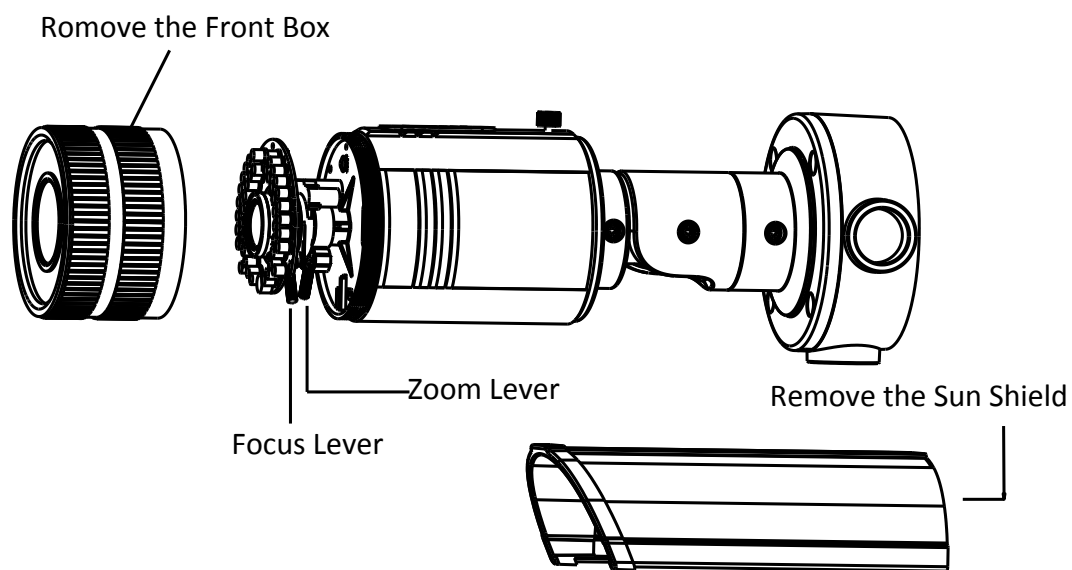
Figure 5-39 Lens Adjustment
