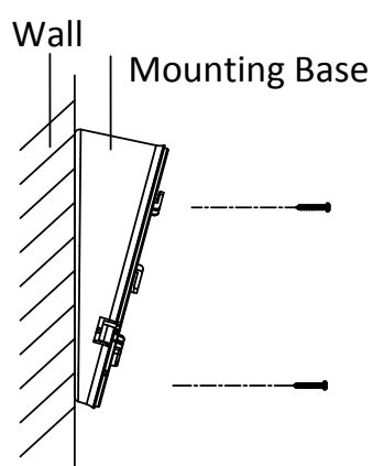
Figure 8-36 Fix the Slant Mounting Base
