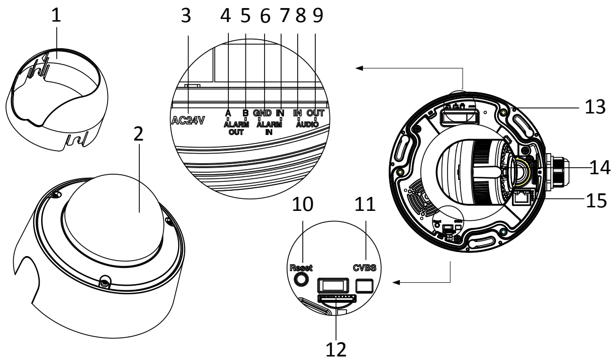
Figure 3-116 Detailed Components
