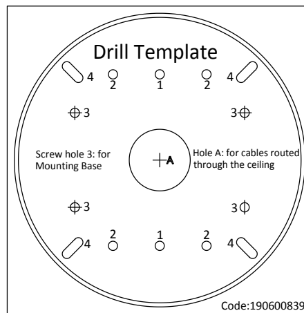
Figure 3-18 Drilling Template
