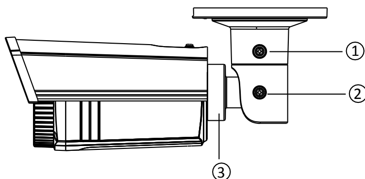
Figure 5-22 3-axis Adjustment
