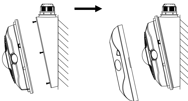
Figure 8-10 Install the Camera Body and Cover
