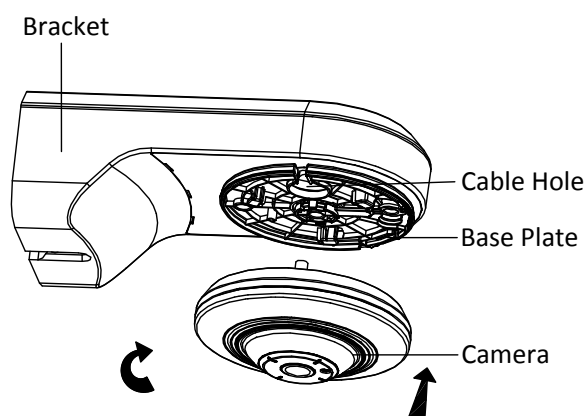
Figure 8-42 Fix the Camera
