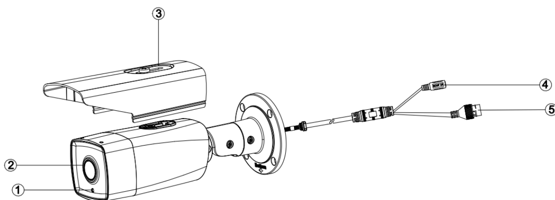
Figure 5-47 Overview
