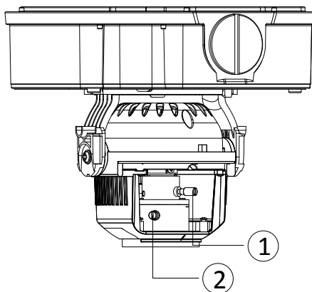
Figure 3-128 Lens Adjustment
