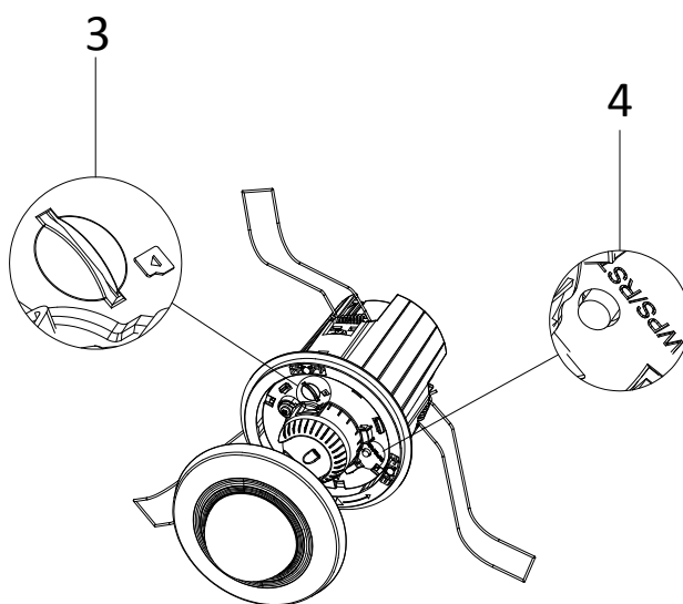
Figure 3-106 Overview(2)
