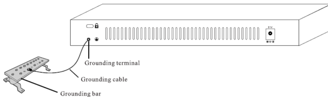
Figure 2.5 Connect to the grounding bar
