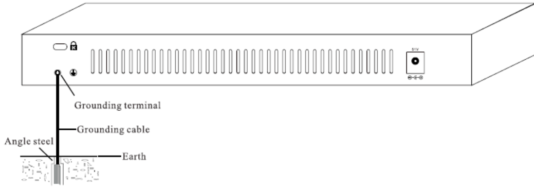
Figure 2.6 Ground with an angle steel
