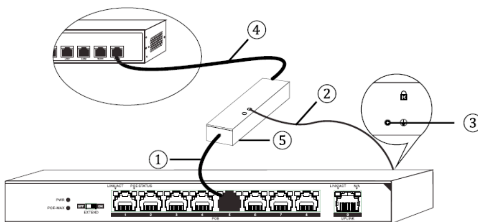
Figure 3.2 Lightning protector connection
