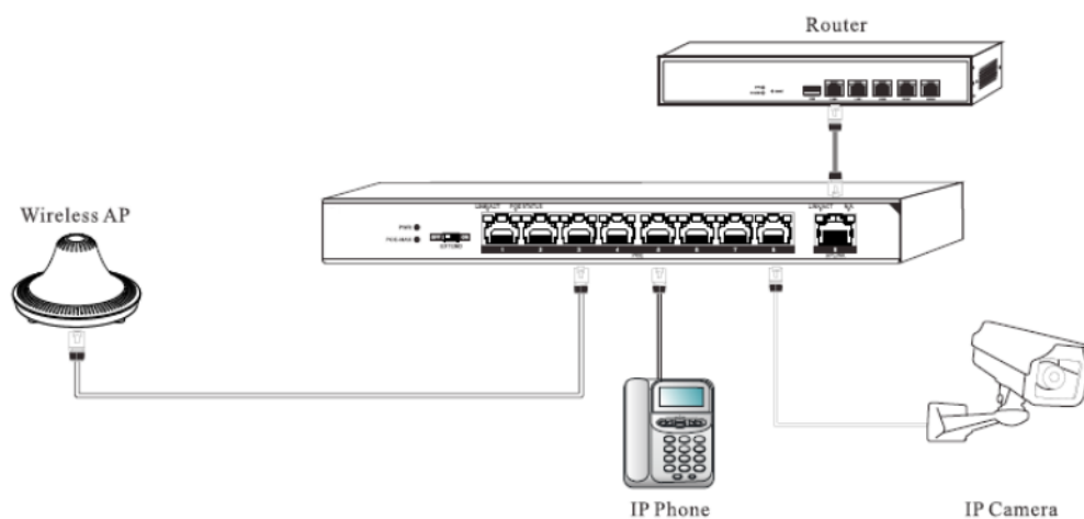
Figure 3.1 RJ45 port connection
