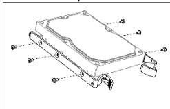
Figure 2-7 Fix Mounting Ear
