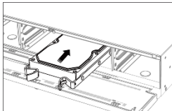
Figure 2-9 Insert HDD
