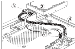
Figure 2-2 Connect Cable
